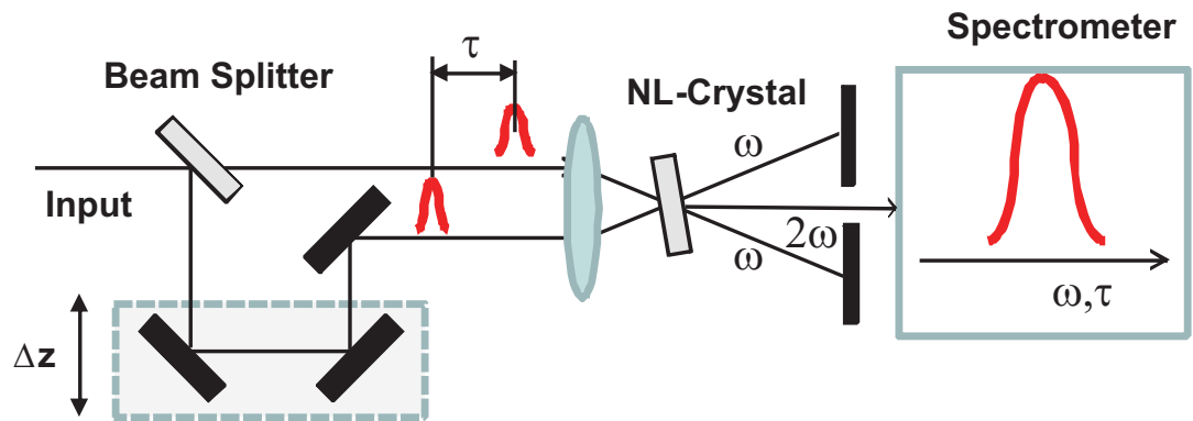
Figure 9.18: SHG-FROG setup.
