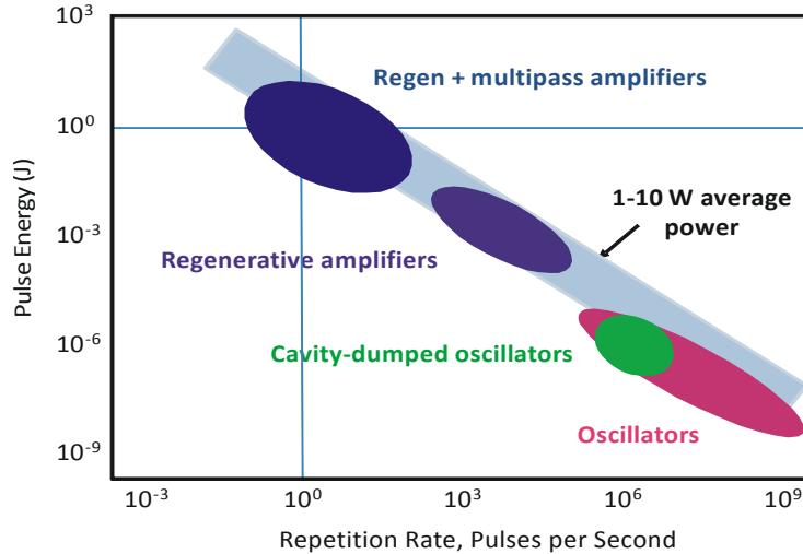
Figure 12.1: Schemes for generating high energy laser pulses.
