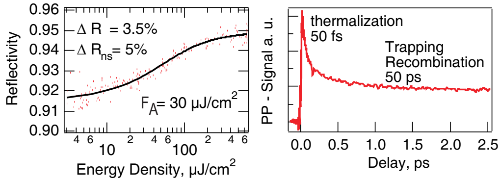
Figure 8.6: Saturation fluence and pump probe measurements with 10 fs pulses on a broadband metal mirror based GaAs saturable absorber. The dots are measured values and the solid line is the fit to a two-level saturation characteristic [11].
