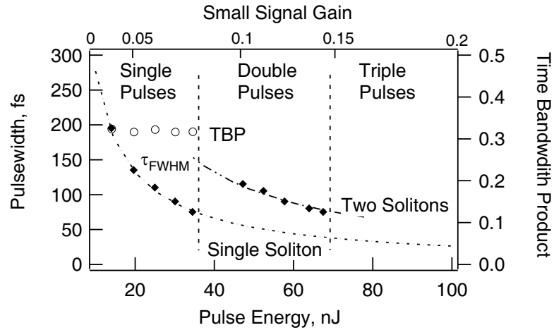
Figure 8.14: Steady state pulse width ( \tau_{FWHM} ) and time-bandwidth product (o) for a Nd:glass laser modelocked by a saturable absorber with a 200 fs recovery time with GDD and SPM included, shown as a function of the intracavity pulse energy. The time-bandwidth product is only meaningful in the single pulse regime, where it is shown. The pulses are almost transform limited sech-pulses. The pulse width in the multiple pulse regime is only unique in the parameter region where multiple pulses of similar height and width are achieved. The pulses break up into multiple pulses when the absorber is about three times saturated.
