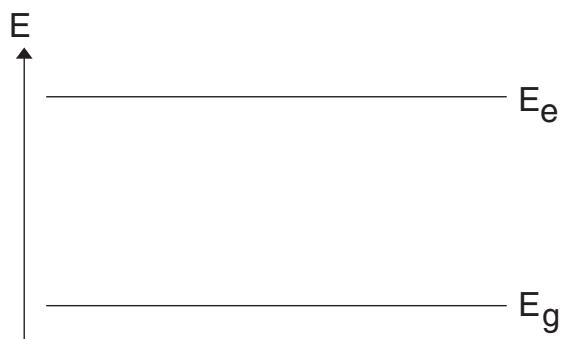
Figure 4.1: Two-level atom
