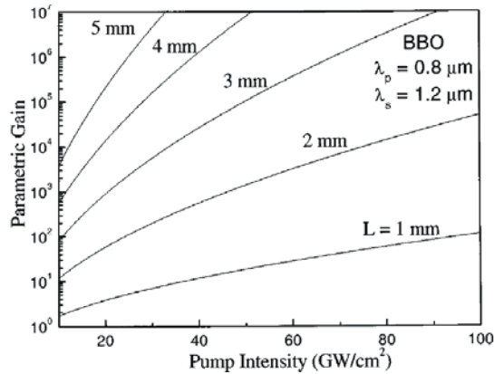
Figure 12.24: Parametric gain for an OPA at the pump wavelength \lambda_p = 0.8 \mu m and the signal wavelength \lambda_s = 1.2 \mu m , using type I phase matching in BBO ( d_{eff} = 2 \text{ pm/V} ). [5]
